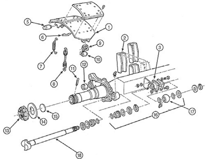
PRO-PAR 5" Square Axle with Brakes HM518445/HM518410 bearing combination for reference only
