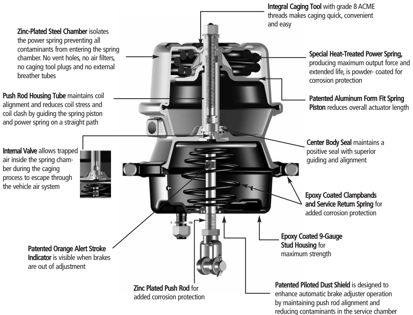
Long Stroke Life Seal® Square ports; trapezoidal shaped tag with stroke information; embossed or "cast-in" service instructions.
