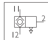
Bendix® QR-1C® Quick Release Valve
